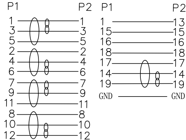
Wiring diagram
