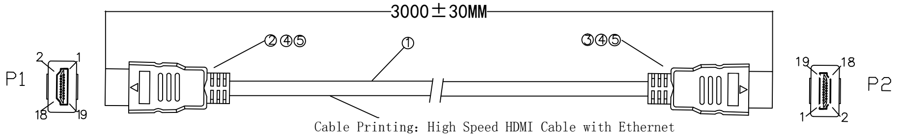
Wiring diagram
